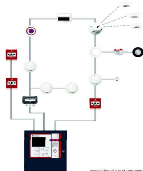
Detector lines of POLON 4100 control panel
