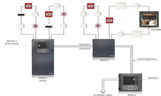
Maximum configuration of distributed control panel:
